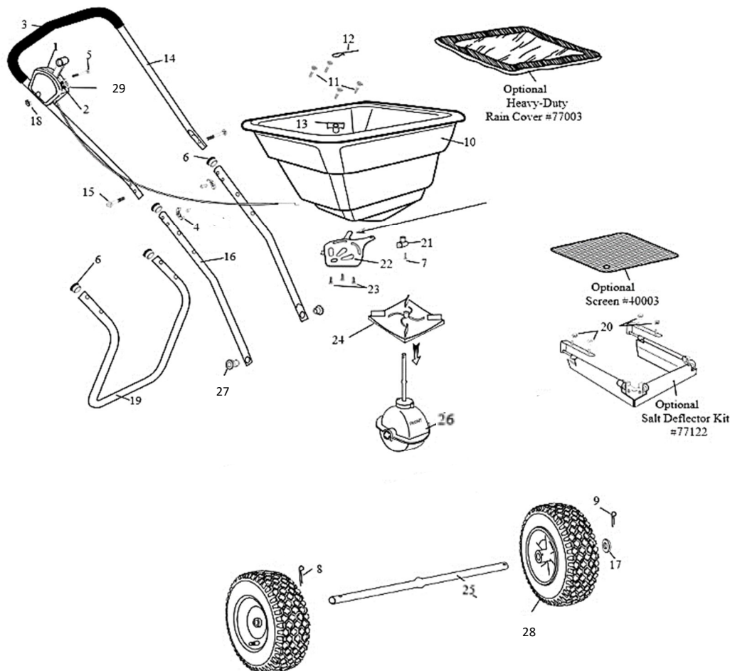
2050P Broadcast Spreader Parts List
